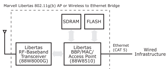
Fig 2. Libertas WLAN 802.11g(b) Access Point Chipset (88W8000G and 88W8510) Applications Diagram
